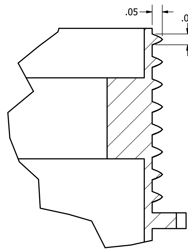
DETAIL C SCALE 4 : 1
